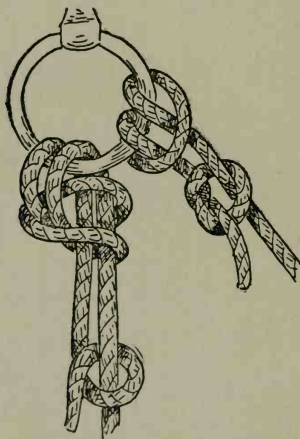
FIG. 56.—Larks' heads and running noose.
